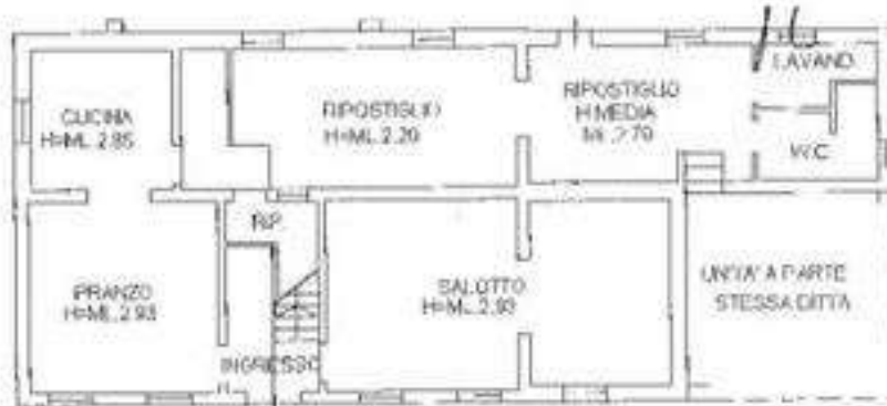
PIANO TERRA
